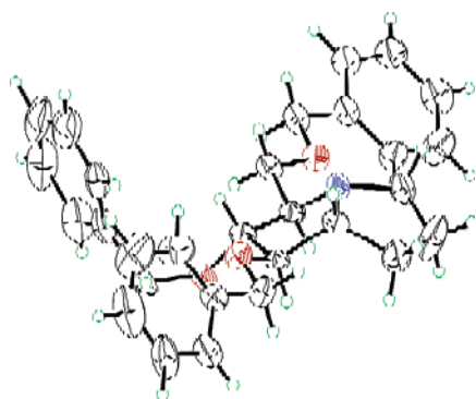
FIGURE 1. ORTEP diagram for compound 11.
